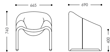
Model: SA260 Size: 665W*690D*740H*400SH
