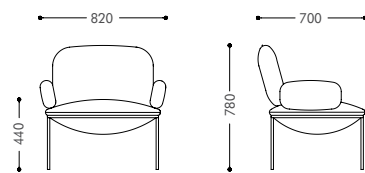
Model: SA255 Size: 820W*700D*780H*440SH
