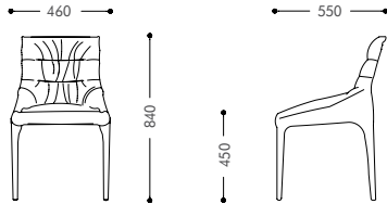
Model: SA269 Size: 460W*550D*840H*450SH
